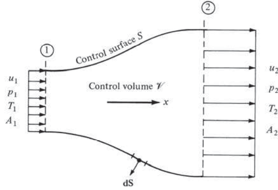
Figure 10.7 Finite control volume for quasi-one-dimensional flow.
