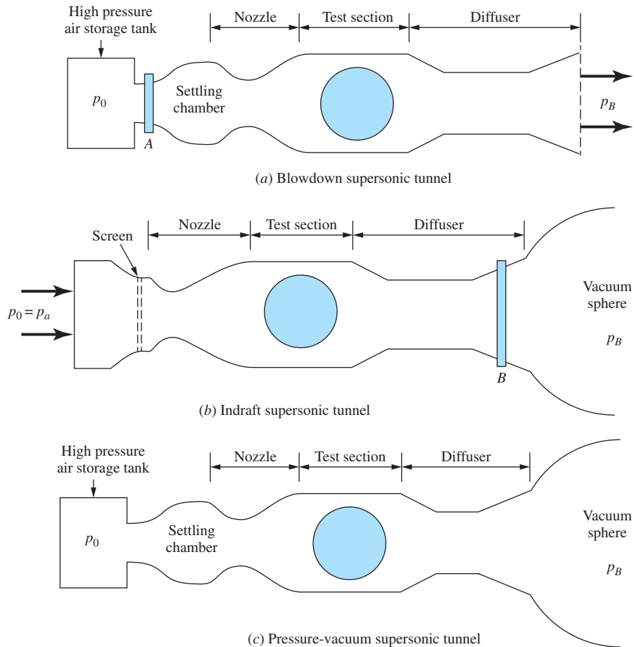
Figure 10.24 Supersonic wind tunnel configurations.
