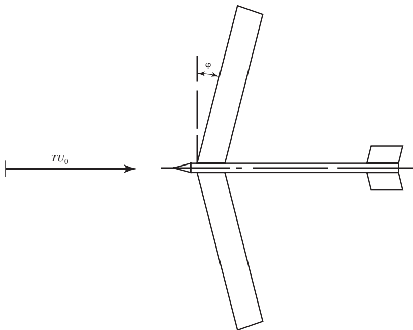
Figure 11.33 A swept-wing airplane planform, from Busemann's original paper in 1935.
