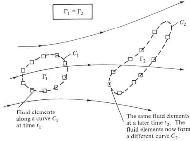
Figure 4.20 Kelvin's theorem.
