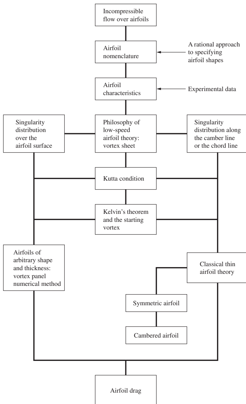
Figure 4.7 Road map for Chapter 4.
