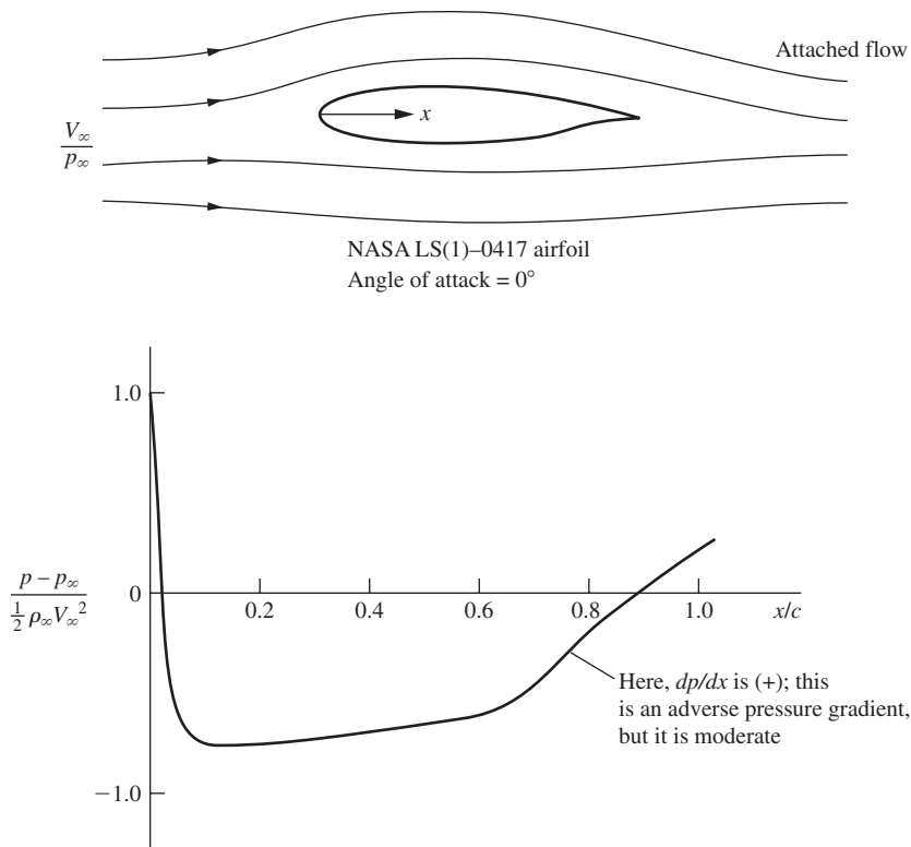
Figure 4.45 Pressure distribution over the top surface for attached flow over an airfoil. Theoretical data for a modern NASA low-speed airfoil, from NASA Conference Publication 2046, Advanced Technology Airfoil Research , vol. II, March 1978, p. 11.
