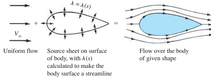
Figure 3.39 Superposition of a uniform flow and a source sheet on a body of given shape, to produce the flow over the body.
