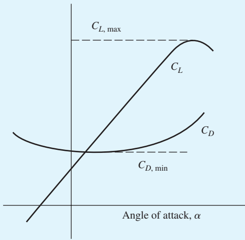
Figure 1.32 Schematic of lift and drag coefficients versus angle of attack; illustration of maximum lift coefficient and minimum drag coefficient.
