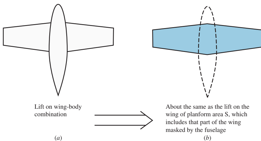
Figure 6.12 Lift on a wing-body combination.
