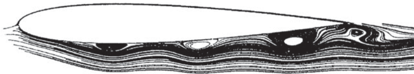
Figure 20.14 Streamline pattern over the bottom of an NACA 0012 airfoil, over which a series of jets is distributed which are alternatively blowing or sucking mass into or out of the flow, with the overall net mass injected into the flow being zero—a zero-mass jet array. (Data Source: Hassan, A. A., and JanakiRam, R. D.: “Effects of Zero-Mass ‘Synthetic’ Jets on the Aerodynamics of the NACA-0012 Airfoil,” AIAA Paper No. 97-2326, 1997).
