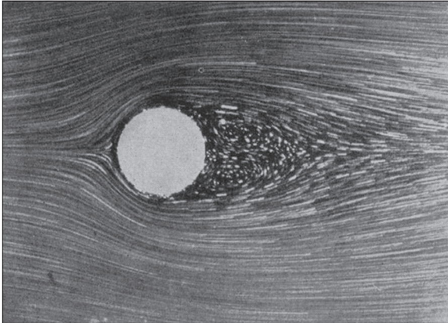
Figure 3.46 Flow over a circular cylinder. Re = 1.54 . (Prandtl, L., and O. G. Tietjens: Applied Hydro and Aeromechanics Based on Lectures of L. Prandtl , United Engineering Trustees Inc., 1934, McGraw-Hill, New York).
