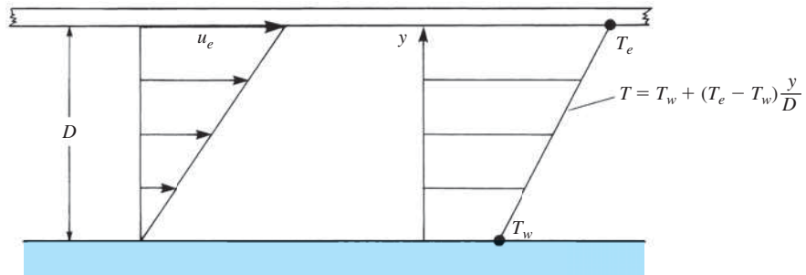
Figure 16.4 Couette flow temperature profile for negligible viscous dissipation.
