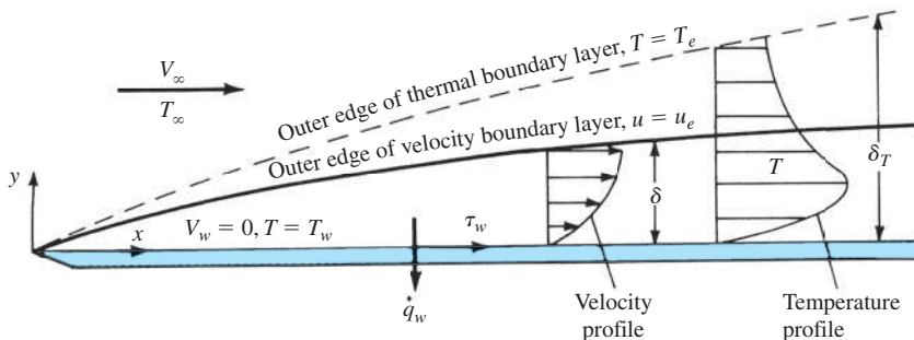
Figure 17.3 Boundary-layer properties.
