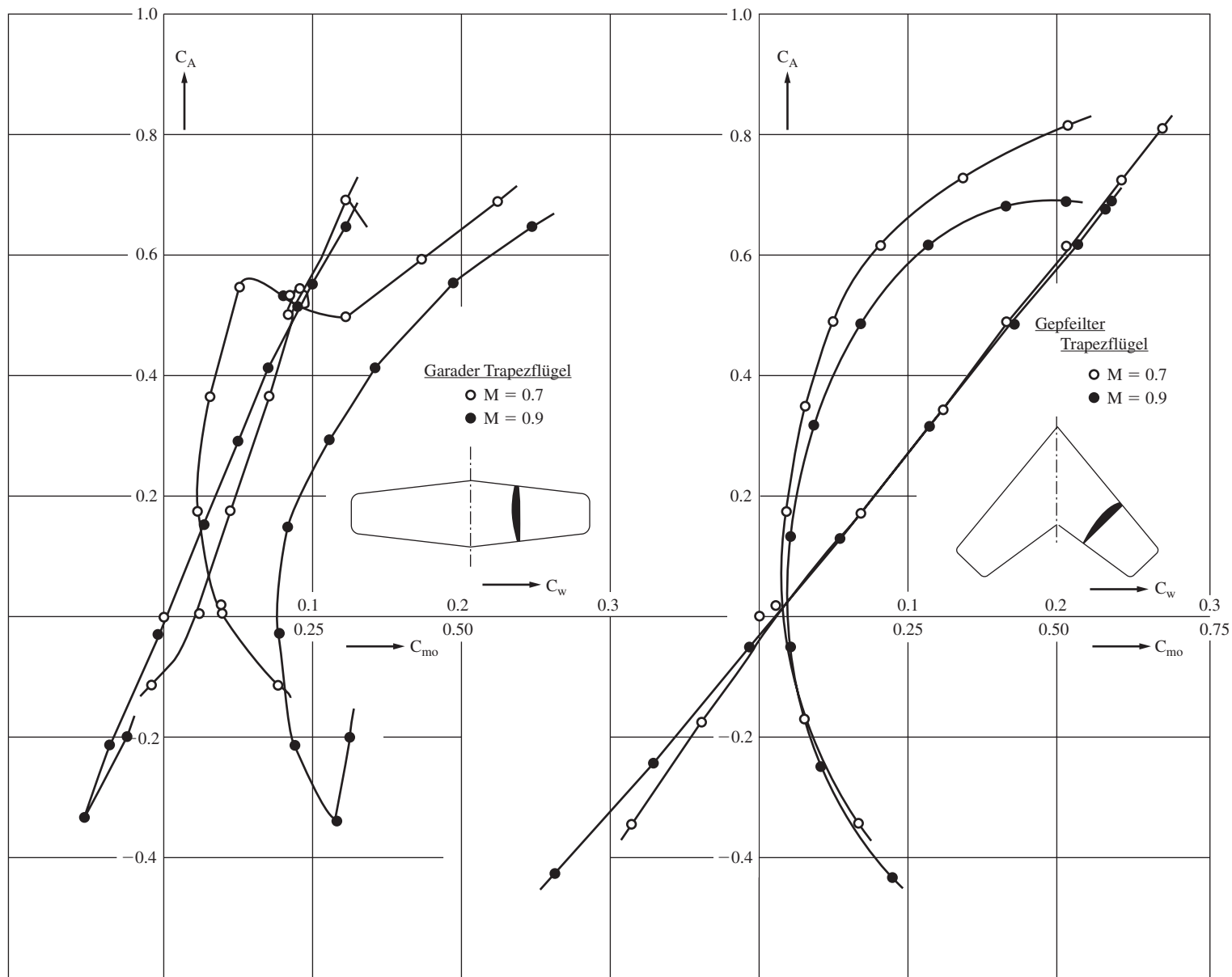
Figure 11.34 Drag polars at Mach 0.7 and 0.9 for a straight wing (left) and swept wing (right), as reported by Ludwig in 1939.
