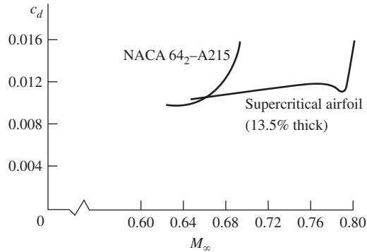
Figure 11.20 The drag-divergence properties of a standard NACA 64-series airfoil and a supercritical airfoil.
