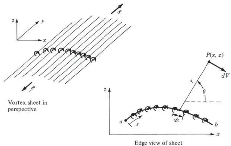
Figure 4.13 Vortex sheet.
