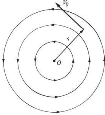
Figure 3.31 Vortex flow.
